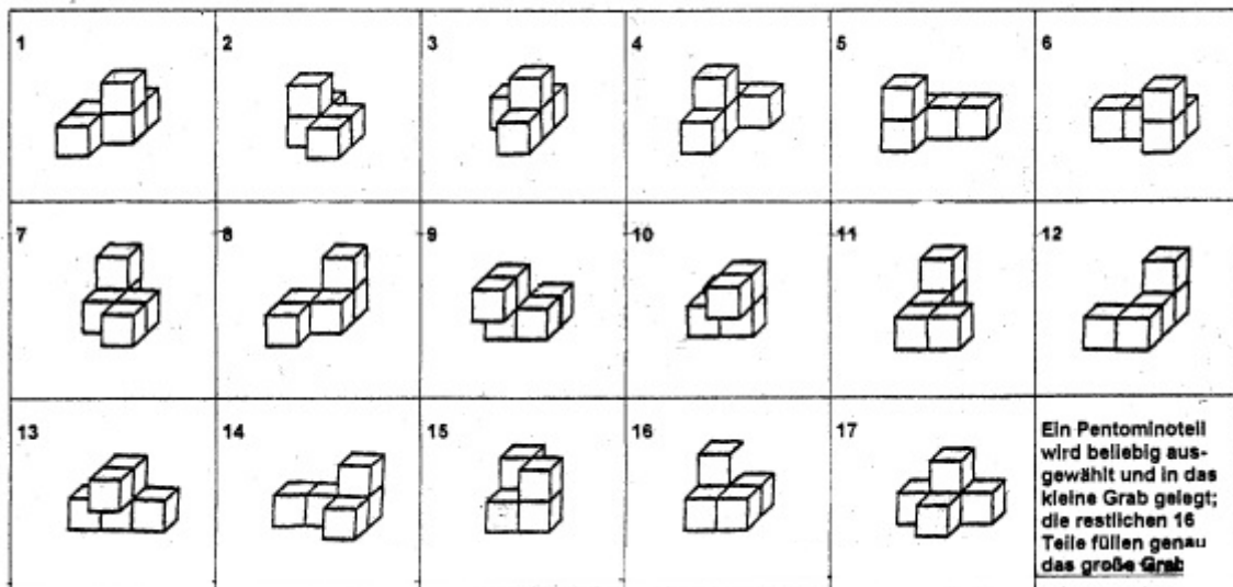
17 nonplanare Pentacuben
